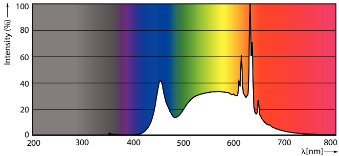
Spectral Power Distribution Colour – MAS LED spot VLE D 2.8-35W GU10 940 36D
