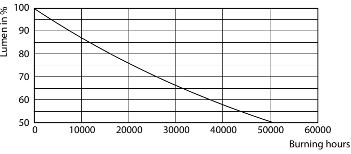
Lumen Maintenance Diagram – MAS LED spot VLE D 2.8-35W GU10 940 36D
