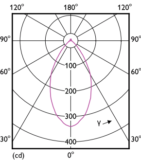
Light Distribution Diagram – MAS LED spot VLE D 3.7-50W GU10 940 60D
