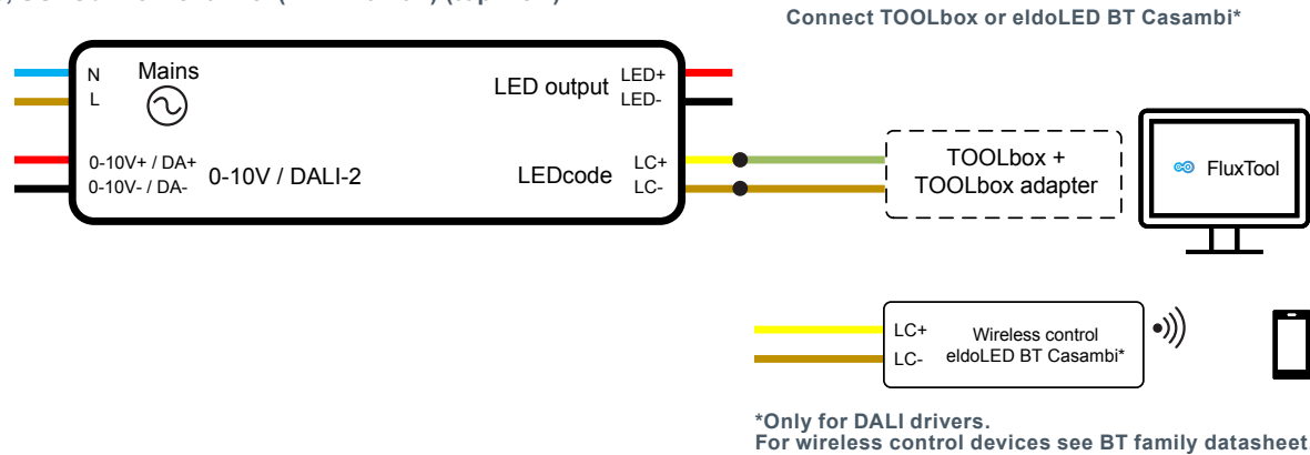
ECODrive, SOLOdrive 1 channel (DALI / 0-10V) (top view)
