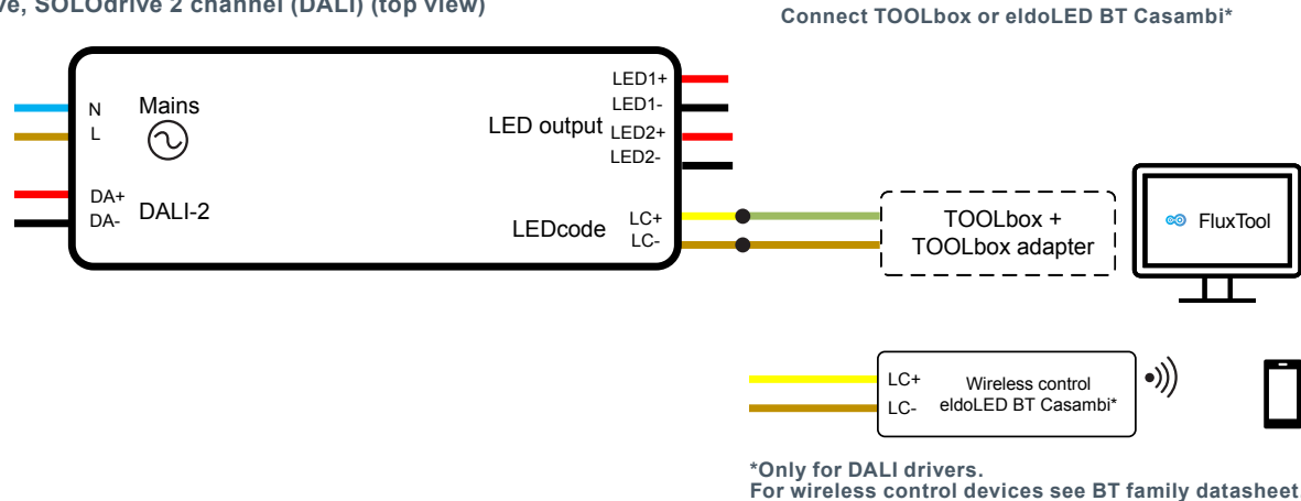
DUALdrive, SOLOdrive 2 channel (DALI) (top view)
