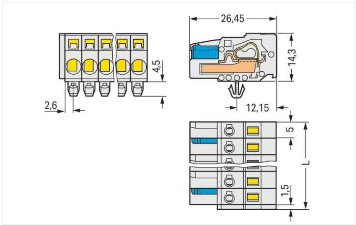
Dimensions in mm L = (\text{pole no.} \times \text{pin spacing}) + 1.5 \text{ mm} 2-pole female connectors – one latch only
