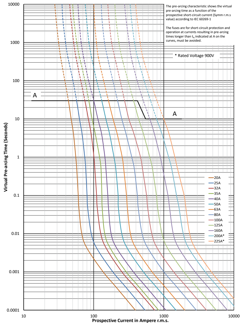
Time-current curve - Size 00, 20 A to 225 A
