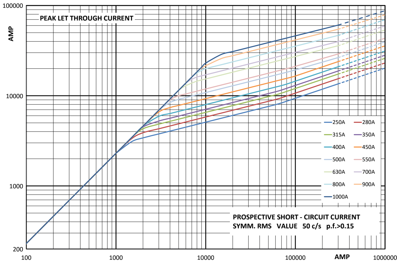
Cut-off curve - Size 2, 250 A to 1000 A
