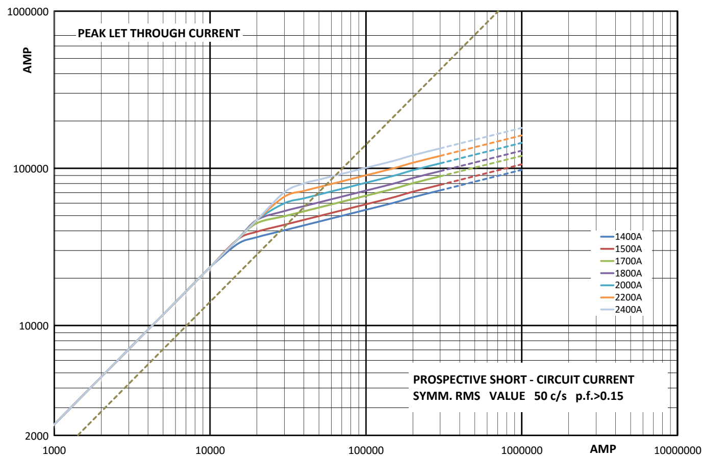
Cut-off curve - 1400 A to 2400 A
