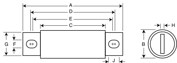
Dimensions (in) - 35 A to 2000 A
