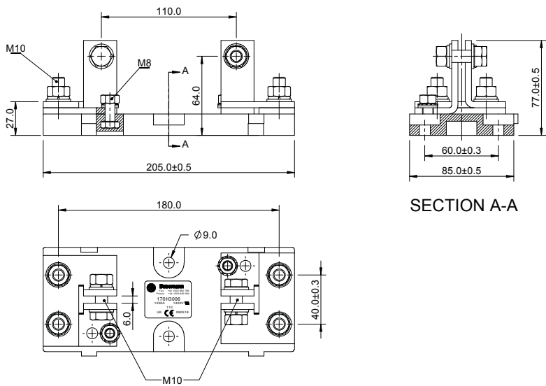
Dimensions (mm) - 170H3006
