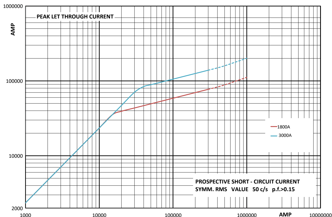
Cut-off curve - IEC Certified fuses - 1800 A and 3000 A
