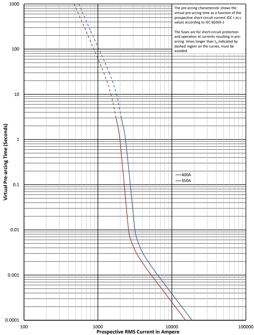
Time-current curve - 350 A and 400 A - 50 mm fuse links
