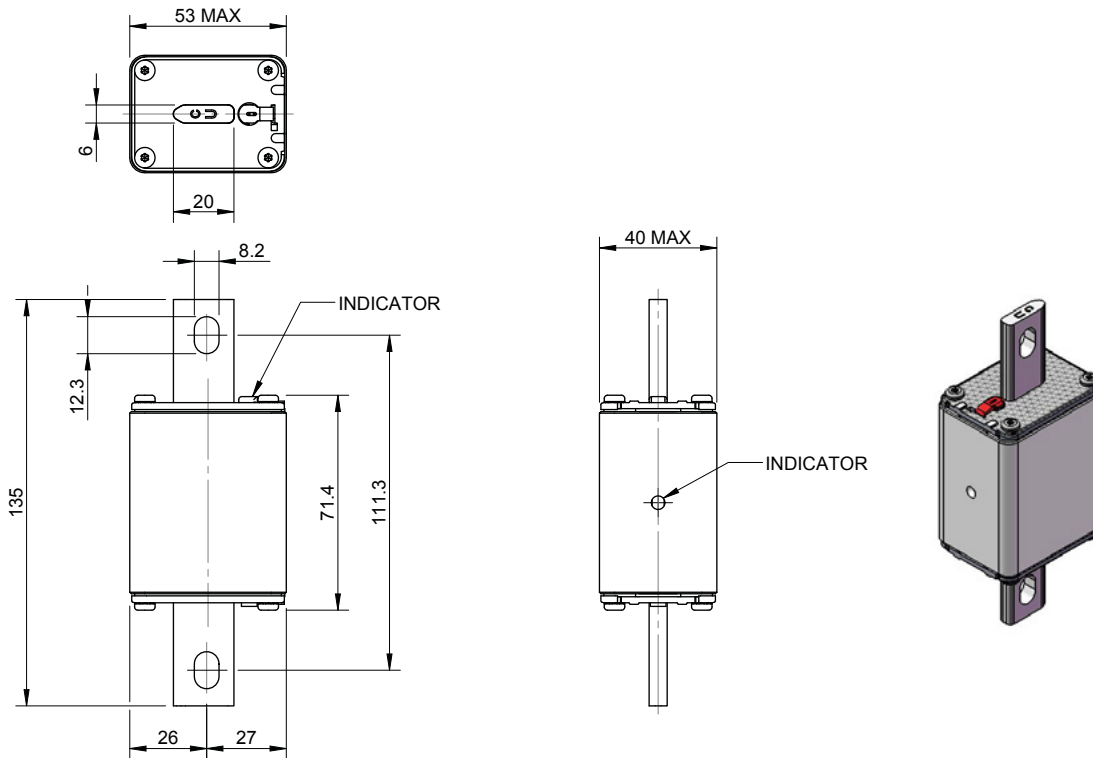
Dimensions (mm) - NH1, blade with bolt holes
