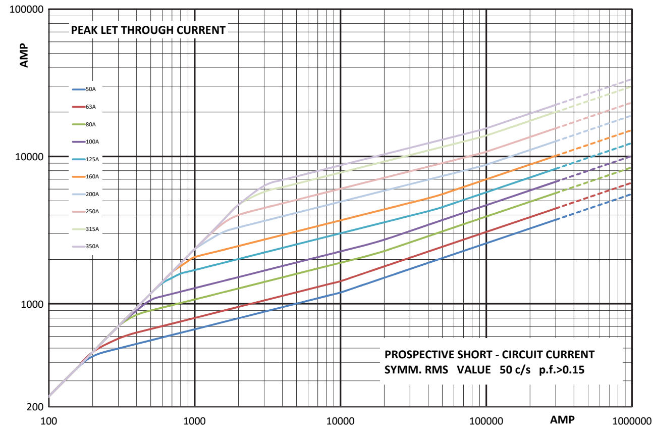
Cut-off curve - Size 1*, 50 A to 350 A
