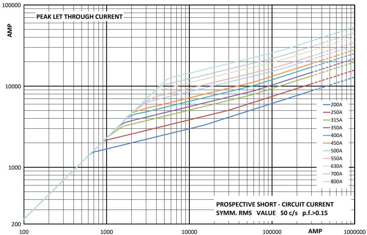
Cut-off curve - Size 1, 200 A to 800 A
