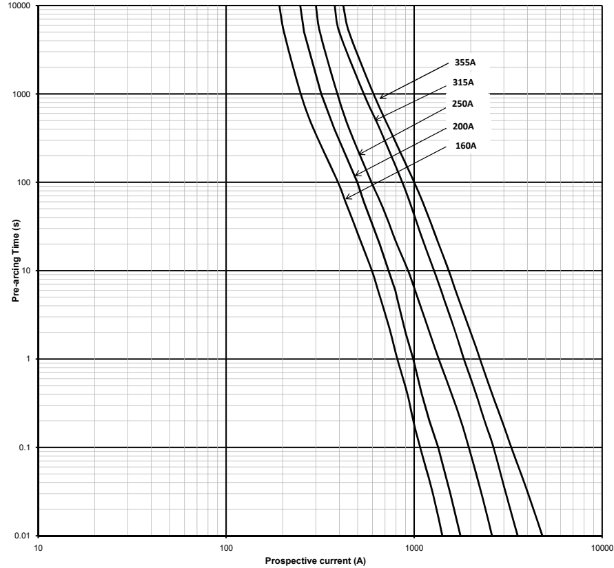
Time-current curve - Size 2XL, bladed and bolted, 1000 V d.c., 160 A to 355 A
