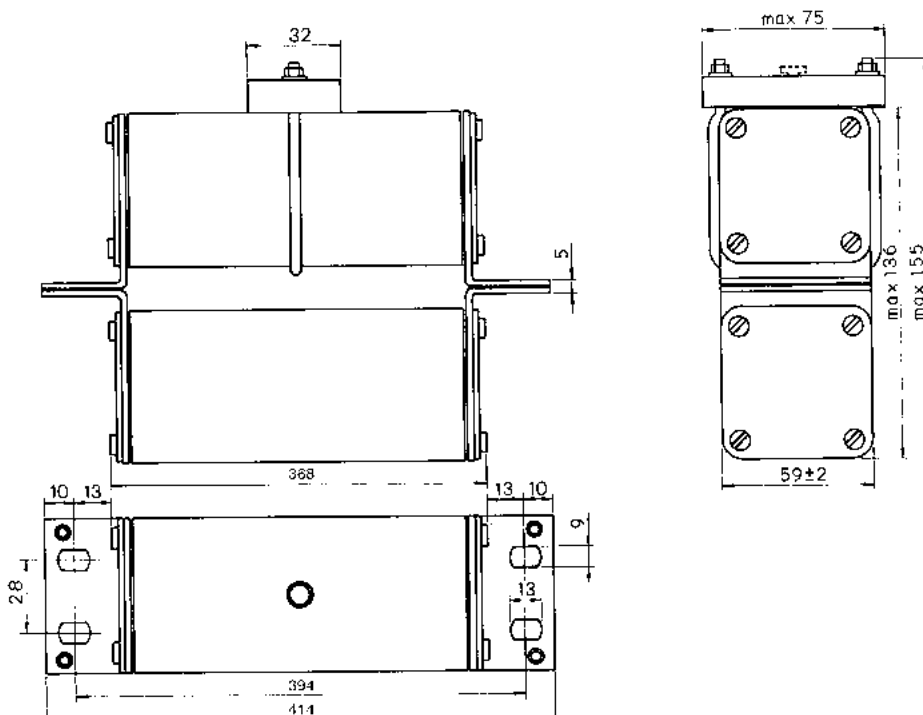
Dimensions (mm) - Size 2//2
