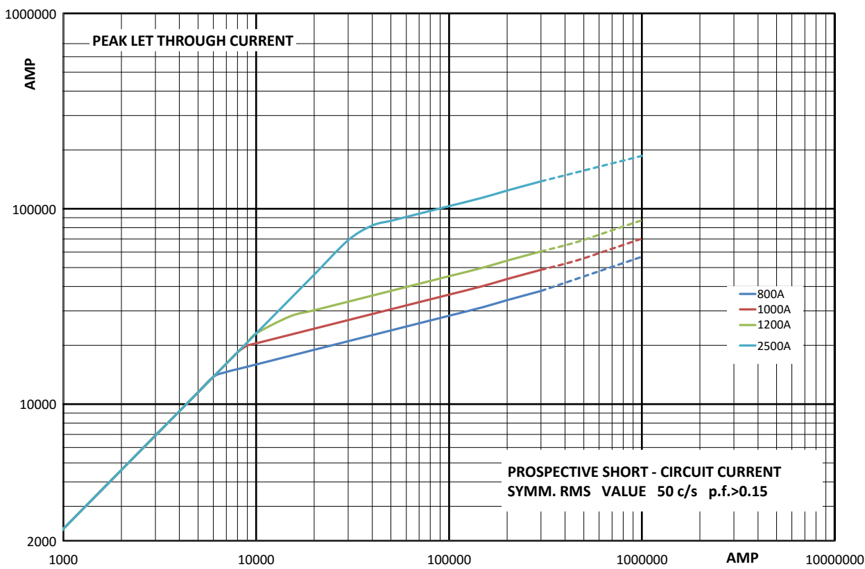
Cut-off curve - 800 A to 2500 A
