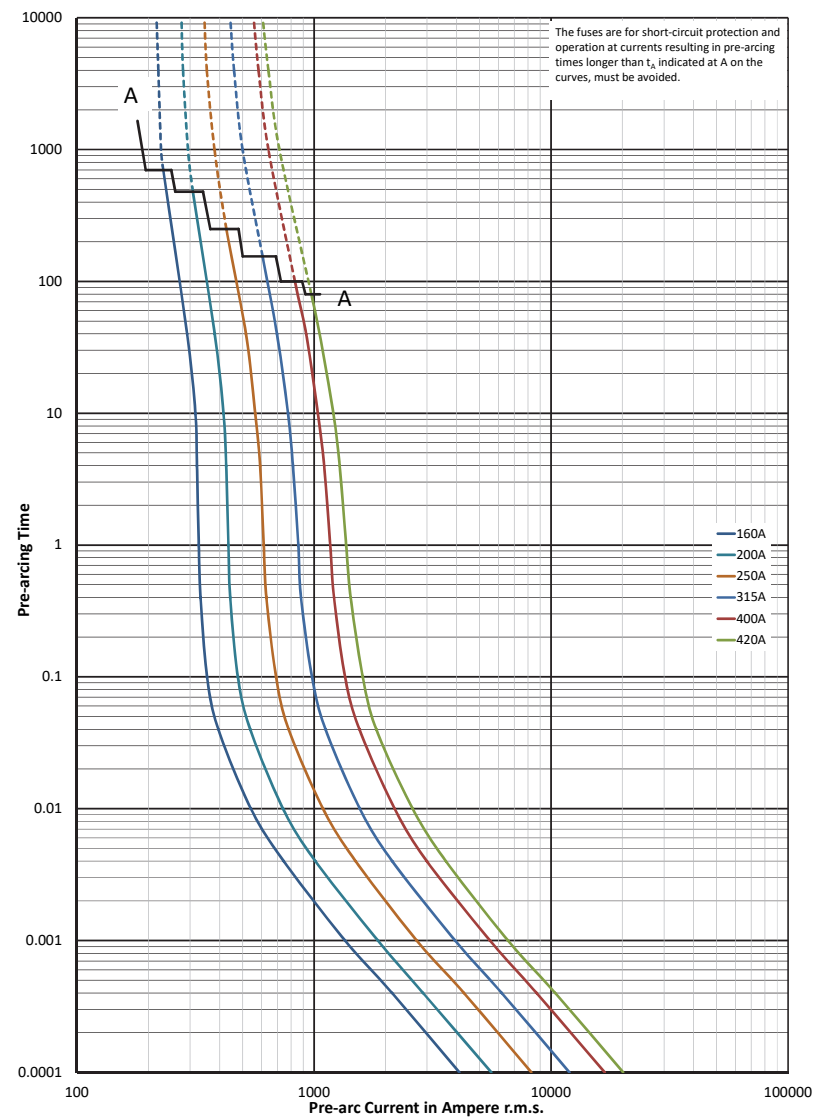
Time-current curve - 160 A to 420 A
