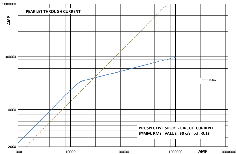
Cut-off curve - 1400 A
