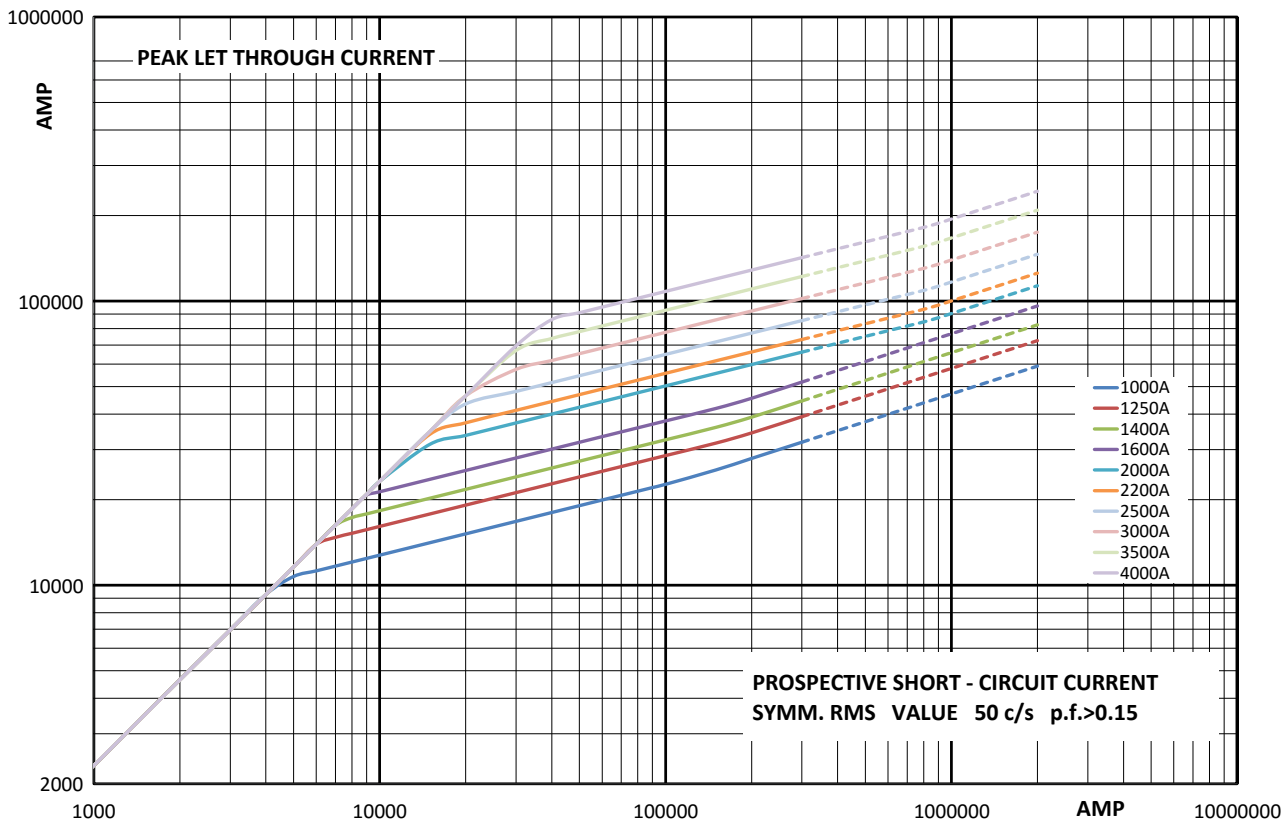
Cut-off curve - 1000 A to 4000 A
