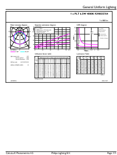
General uniform lighting - CorePro LED PLT HF 6.5W 840 4P GX24q-2
