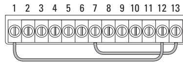
Figure 77: STO control signal terminals (direct enable)
