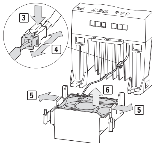
Figure 22: Release the plug connection
