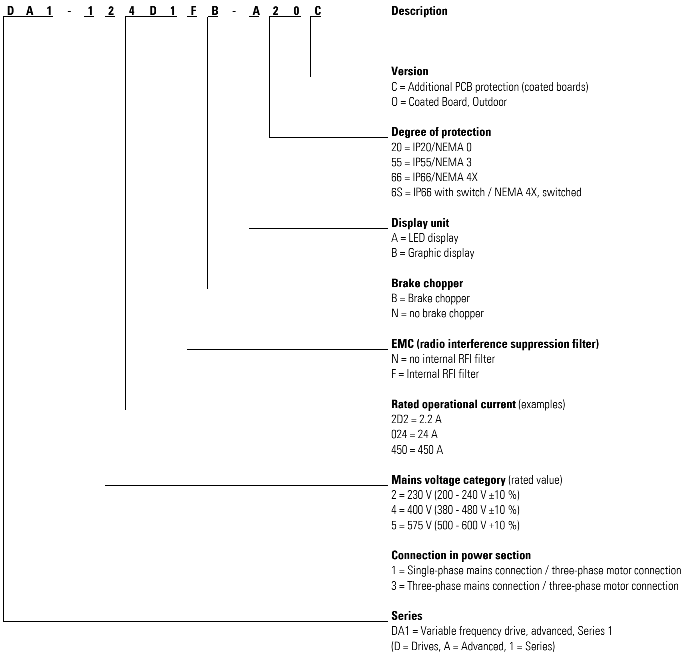
Figure 7: Type code
