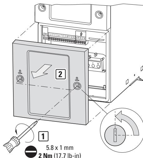
Figure 60: Removing the cover
