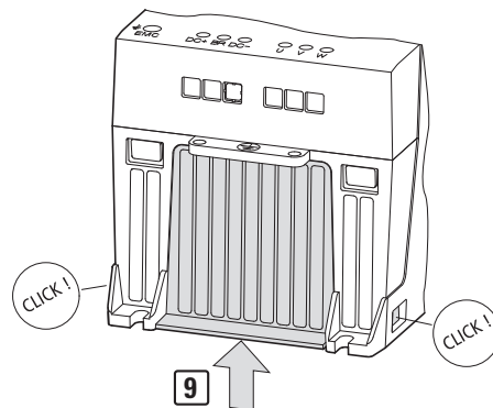
Figure 24: Reinsert the fan cover
