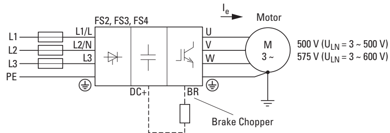
Figure 18: DA1-35...NB-... (without radio interference suppression filter)
