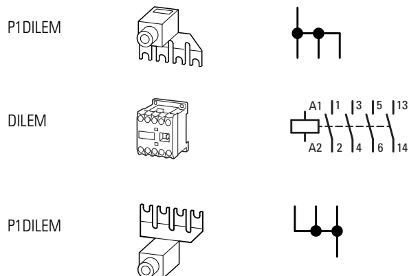
Figure 95: Mains contactor at single-phase connection (DA1-12...)
