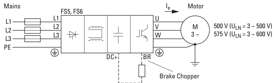
Figure 19: DA1-34...NB-B55C with DC link choke (without radio interference suppression filter)
