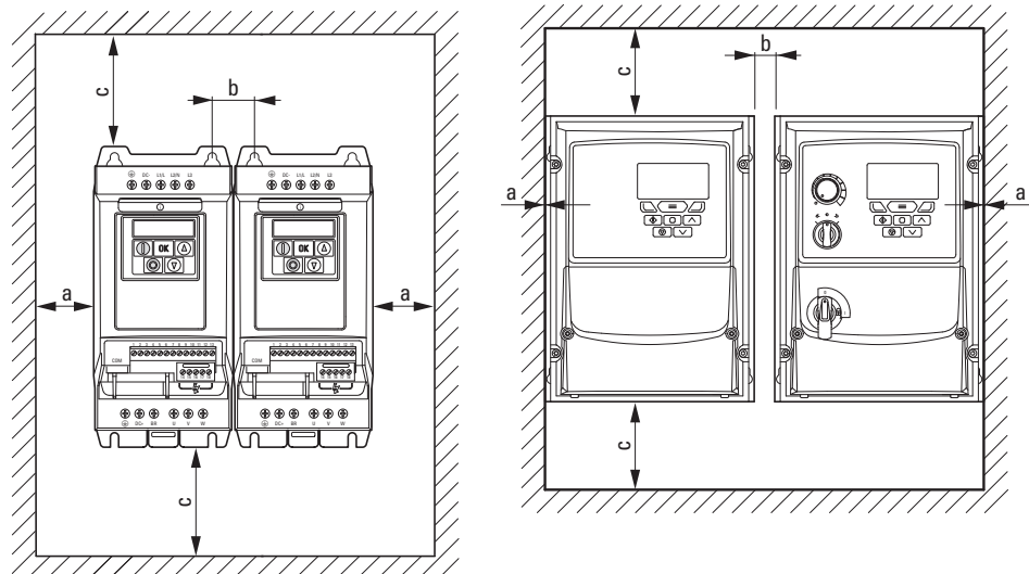
Figure 42: Clearances for air cooling (left: IP20; right: IP66)
