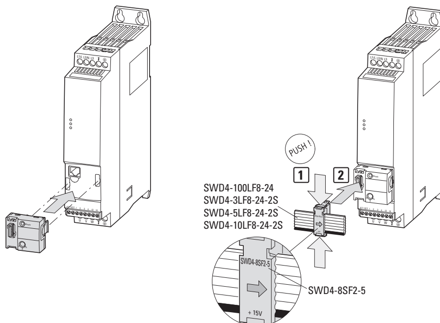
Figura 80: Conectarea SmartWire-DT
