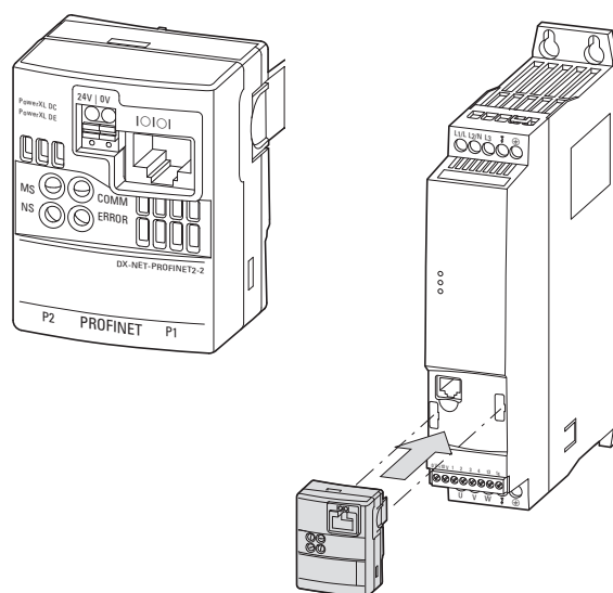
Figura 61: DX-NET-PROFINET2-2 Modulo PROFINET
