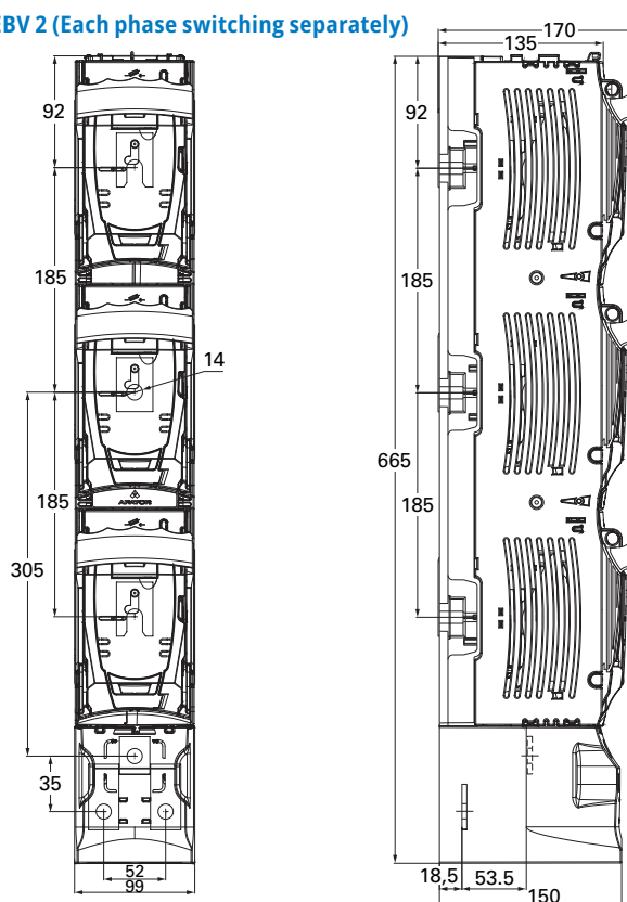
M12 Screws
