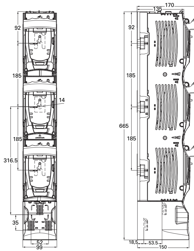
V-Terminals
