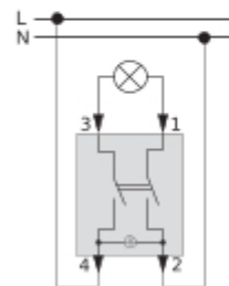
One-way switch 2 pole with indicator light Mxx3x02-0000
