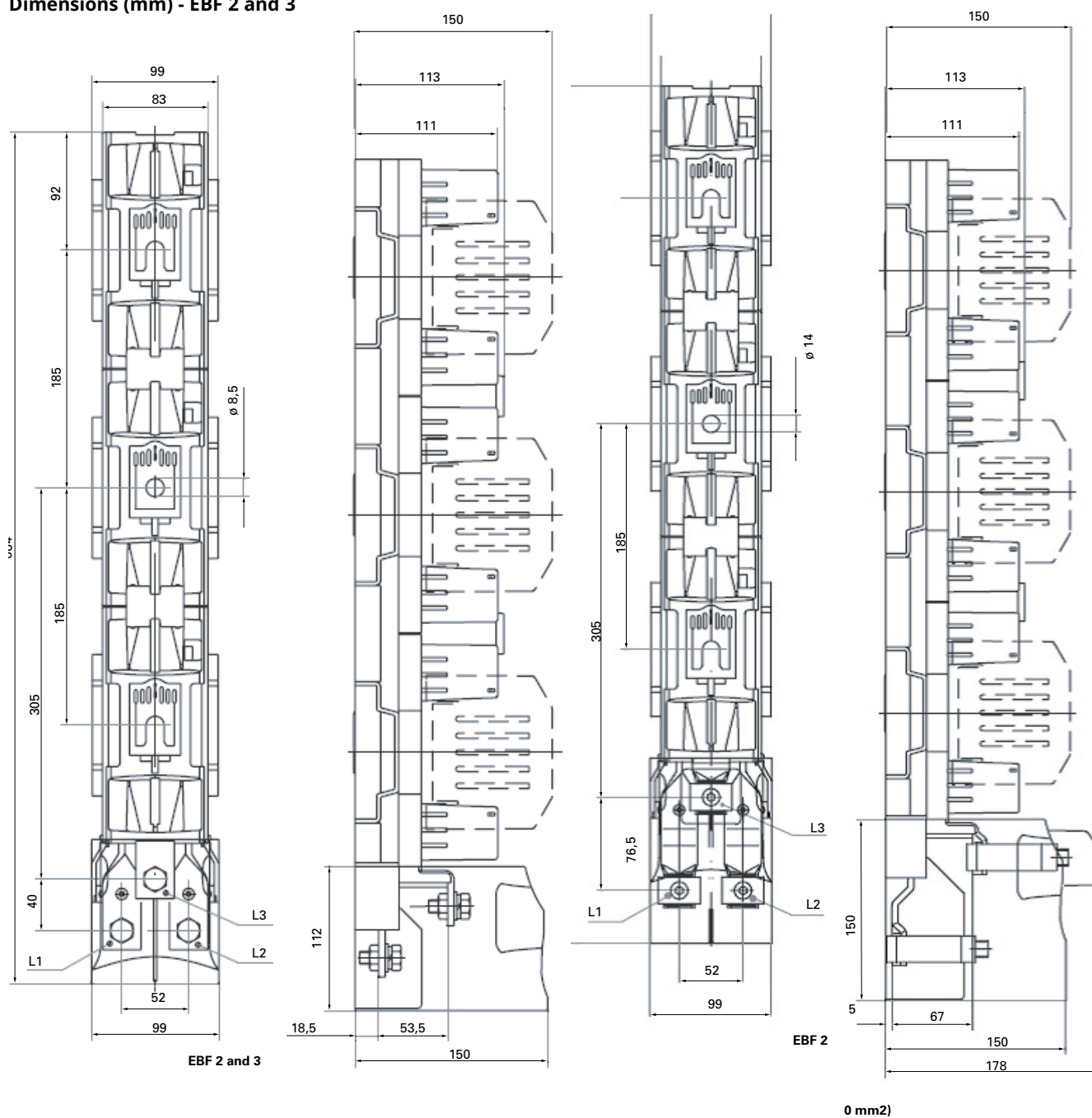
EBF 2 and 3 With terminals 2V (2 x 240 mm 2 )
