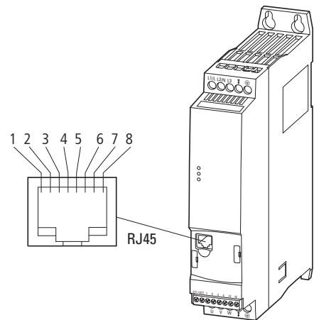
Figura 54: Interface RJ45
