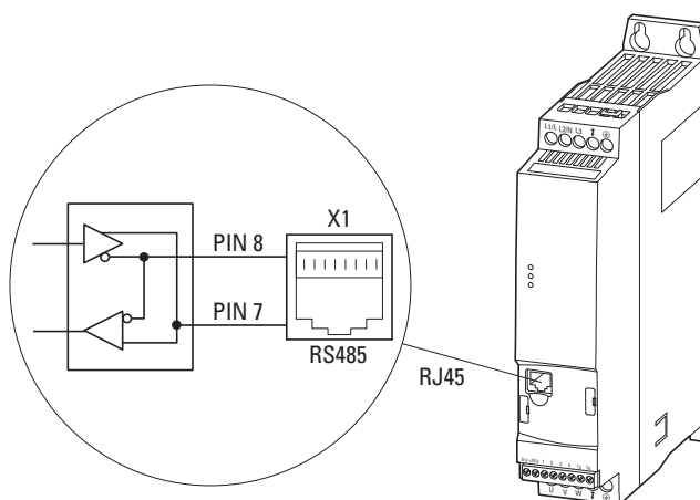
Figura 43: Interface RJ45
