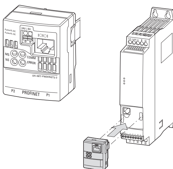
Figura 61: DX-NET-PROFINET2-2 Módulo PROFINET
