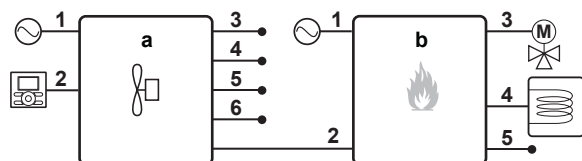
a Buitenunit b NHY2KOMB28+32AA gasboiler
