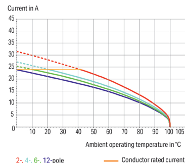
Derating Curve 2-conductor female connector (231-2202/026-000) with THT male header (231-262/001-000) Pin spacing: 7.5 mm / Conductor cross-section: 2.5 mm 2 *f-st* Based on: EN 60512-5-2 / Reduction factor: 0.8
