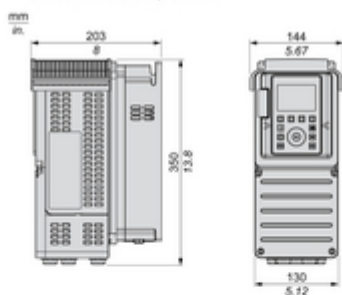
Drives With IP21, Top Cover
