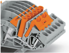
Jumper with safety lid Longitudinal switching disconnect terminal blocks with inserted jumper, including safety lid
