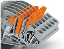
Jumper with safety lid Jumper in pre-locked position
