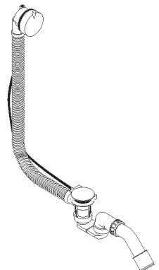
Flexaplusthrough 58150XX0
