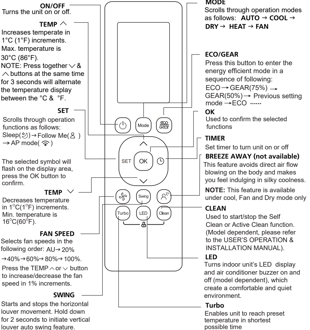
Model: RG10A(D2S)
