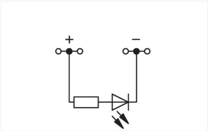
Component terminal block with led, 280 Series, gray
