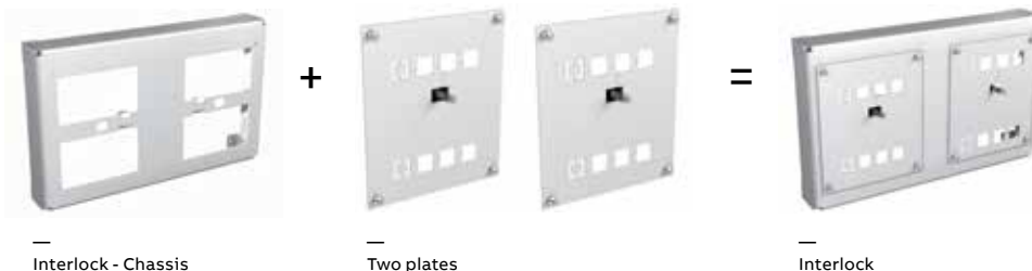
Interlock - Chassis
