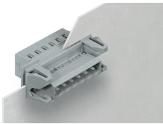
Male connector, with snap-in flanges, for feedthrough applications, for 0.5 ... 2.5 mm plate thickness
