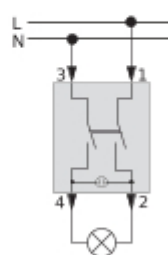
One-way switch 2 pole with indicator light Mxx3x02-0000
