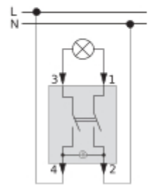
One-way switch 2 pole with indicator light Mxx3x02-0000
