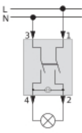
One-way switch 2 pole with indicator light Mxx3x02-0000
