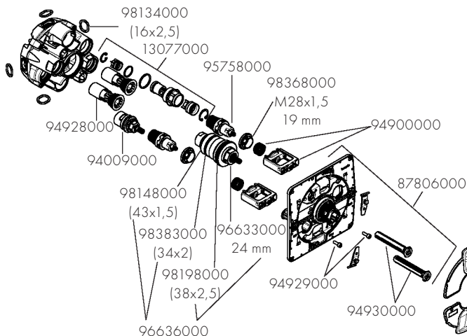
AXOR ShowerSelect ID round 36751XX0 / 36747140 / 36766140
