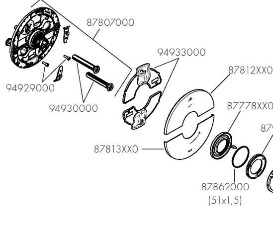
AXOR ShowerSelect ID round 36751XX0 / 36747140 / 36766140
