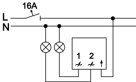
Fig 2: Circuit diagram
