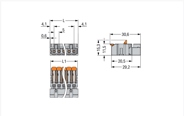
Dimensions in mm L1 = (\text{pole no.} \times \text{pin spacing}) + 3.2 \text{ mm} L2 = (\text{pole no.} \times \text{pin spacing}) + 2 \text{ mm}
