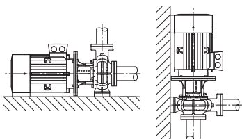
Fig. 15: CronoBloc-BL-E
