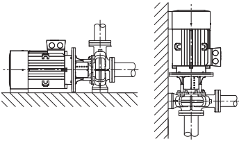
Fig. 15: CronoBloc-BL-E
