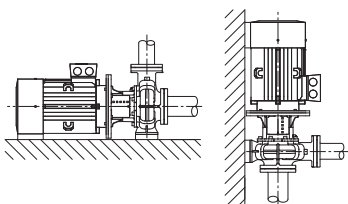
Fig. 15: Wilo-CronoBloc-BL-E
