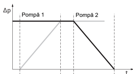
Fig. 11: Alternarea pompelor, schematic
