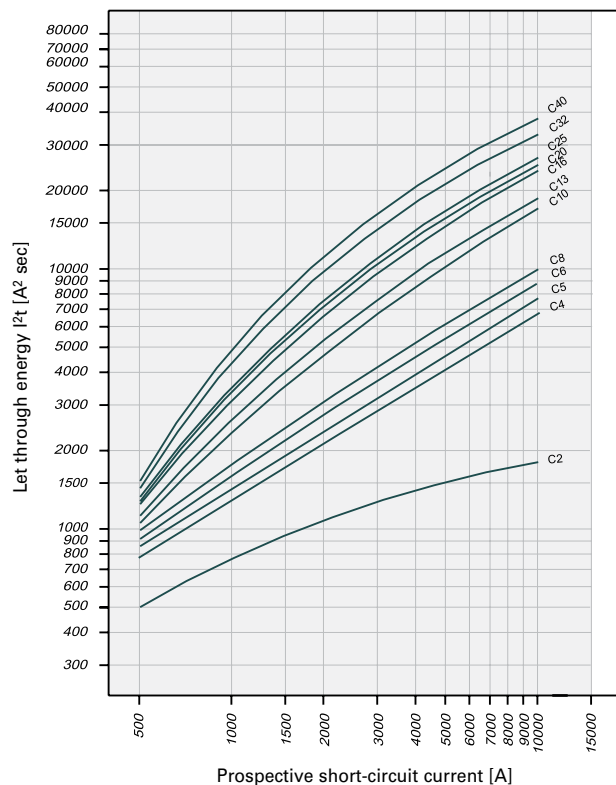
Let-through Energy PKNM, Characteristic C, 1+N-pole
