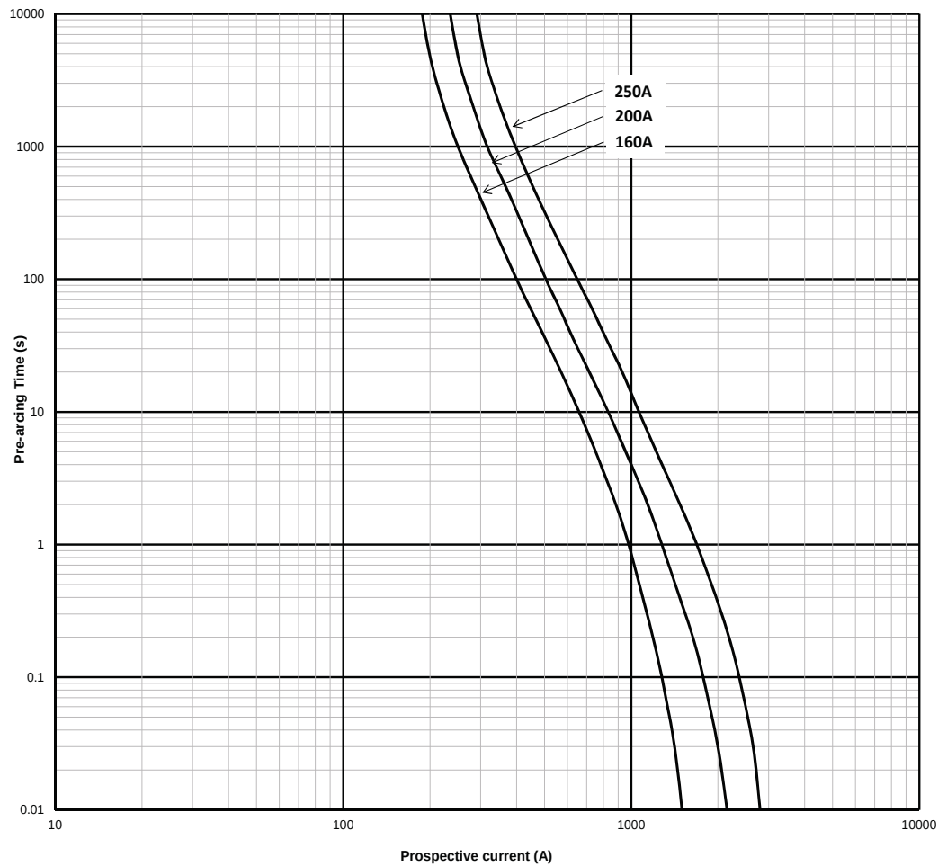
Time current-curve - Flush end
