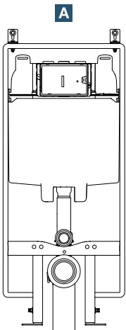
Prosys 80 | Mechanic
