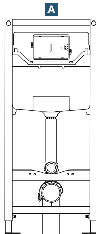
Prosys 120 | Mechanic
