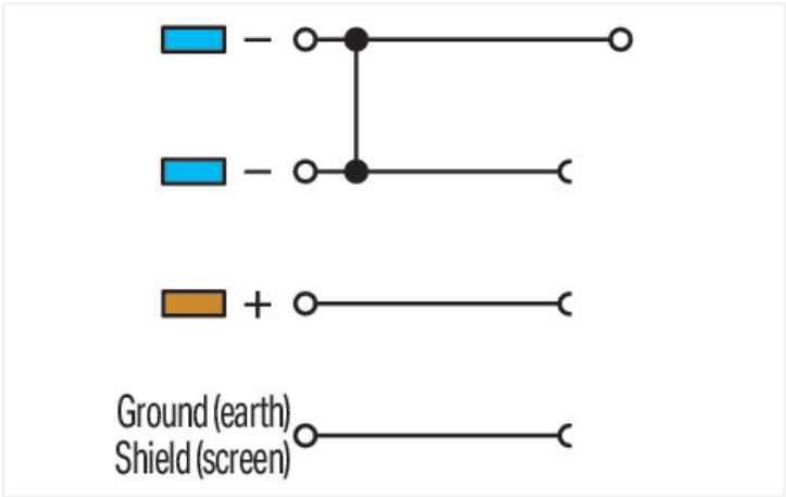
Sensor terminal block, 270 Series, orange
