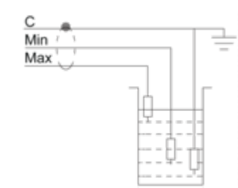
Wiring Diagram
