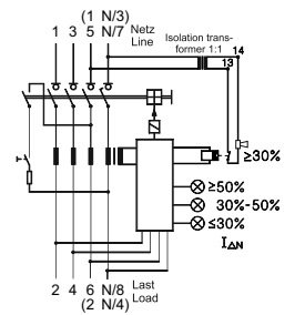
③ Signalisation with Isolation Transformer 1:1 (IEC/EN 60664)
