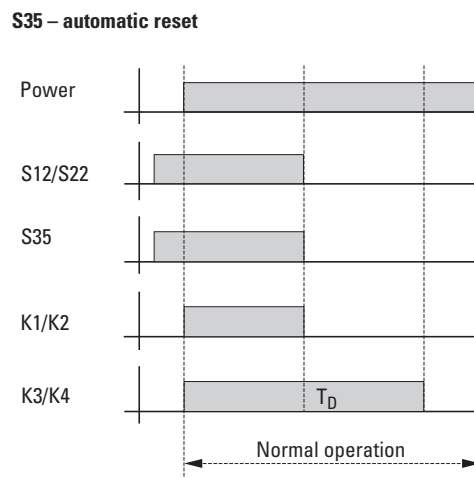
Figure 7: Automatic reset
