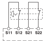
Figure 8: Cross-circuit monitoring
