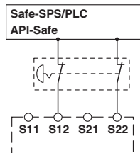
Figure 10: Cross-circuit monitoring via external clock signals
