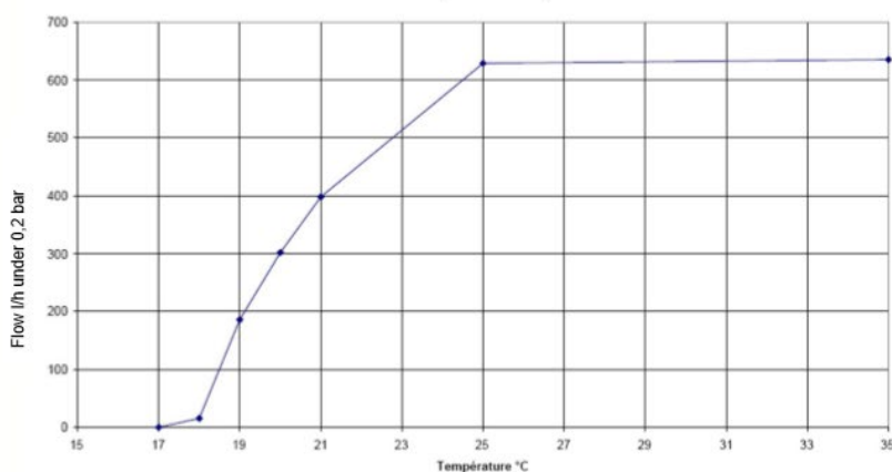
Flow vs Temperature diagram
