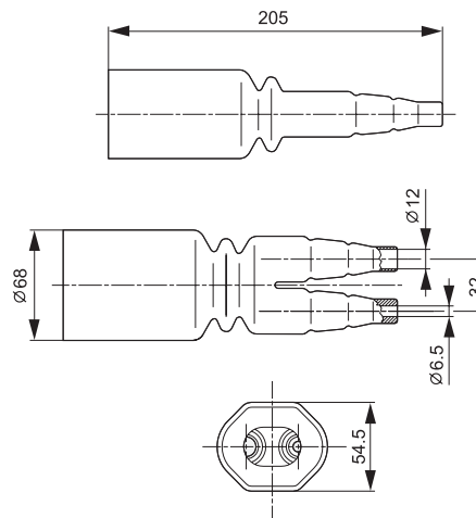
Cable separation ASPIFT23CS
