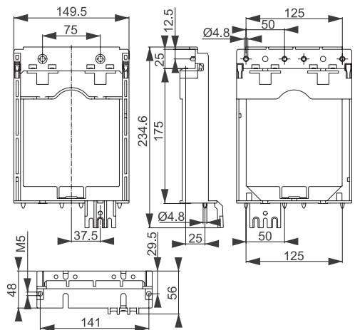
Terminal guide-rail ASPIFT23SG
