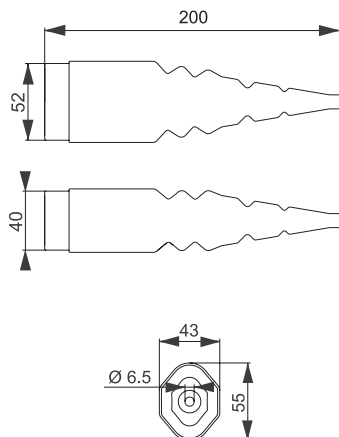
Cable separation ASPIFT1CS
