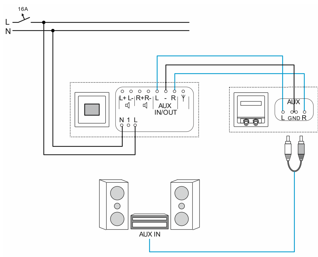
Fig. 91: Flush-mounted radio with HiFi system: Overview
