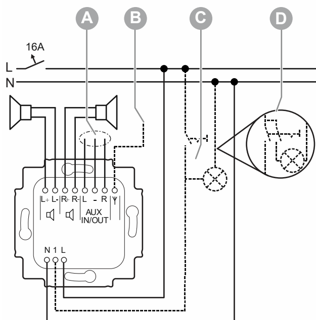
Fig. 8: Electrical connection
