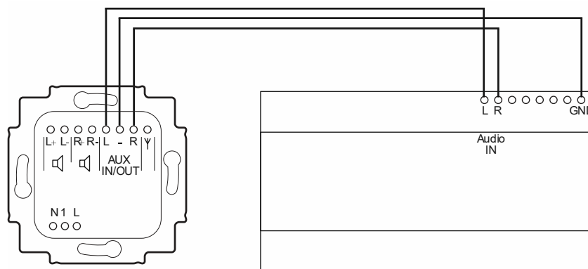
Fig. 12: AUX connection of an amplifier
