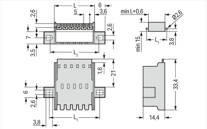
Dimensions in mm L = (\text{pole no.} \times \text{pin spacing}) + 2.2 \text{ mm} L1 = (\text{pole no.} \times \text{pin spacing}) + 8 \text{ mm} L2 = (\text{pole no.} \times \text{pin spacing}) + 7 \text{ mm}
