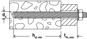
Anchor rod FIS A: Application in concrete
