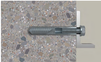
fischer internal threaded rod RG M I
