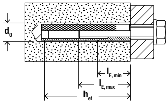
Internal threaded anchor FIS E: Application in solid masonry, perforated brick masonry and aerated concrete
