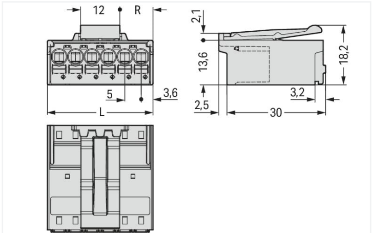
Dimensions in mm L = (pole no. x pin spacing) + 2.2 mm Even pole number R = (L – 12 mm) : 2 Odd pole number R = (L – 17 mm) : 2
