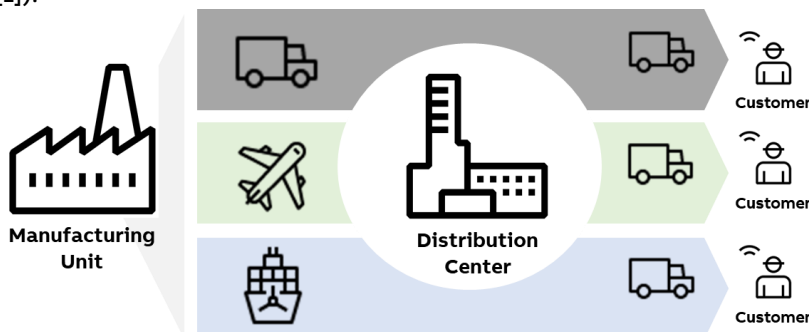
Figure 2: Distribution methodology.
