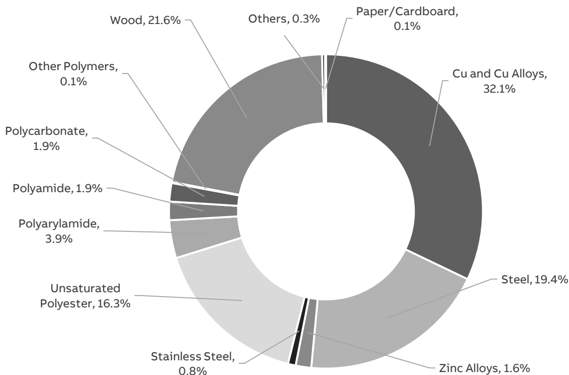
Figure 1: Composition of OTM2000E4CM230C
