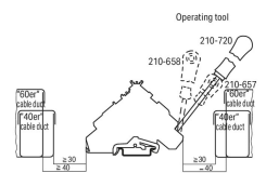
Min. mounting distance – terminal blocks to cable duct
