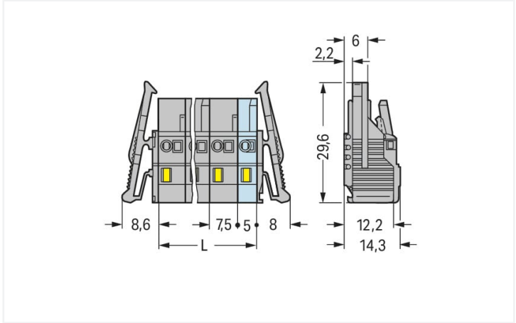
Dimensions in mm L = (pole no. – 1) x pin spacing + 5 mm 2- to 3-pole female connectors – one latch only
