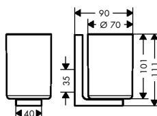
AXOR Universal Rectangular 42604XX0
