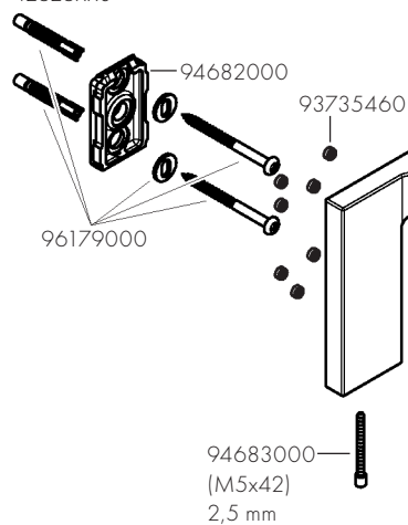
AXOR Universal Rectangular 42626XX0
