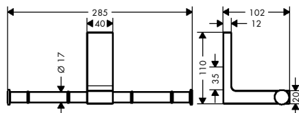
AXOR Universal Rectangular 42657XX0
