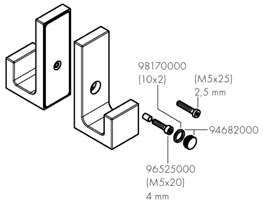
AXOR Universal Rectangular 42639XX0
