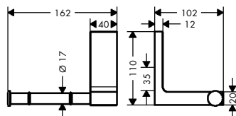
AXOR Universal Rectangular 42656XX0
