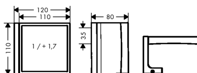
AXOR Universal Rectangular 42649XX0
