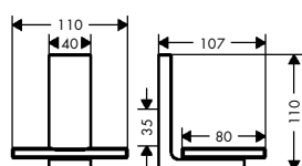
AXOR Universal Rectangular 42605XX0
