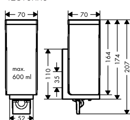
AXOR Universal Rectangular 42610XX0
