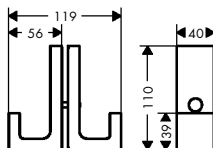
AXOR Universal Rectangular 42639XX0
