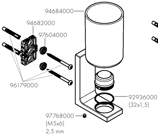
AXOR Universal Rectangular 42610XX0
