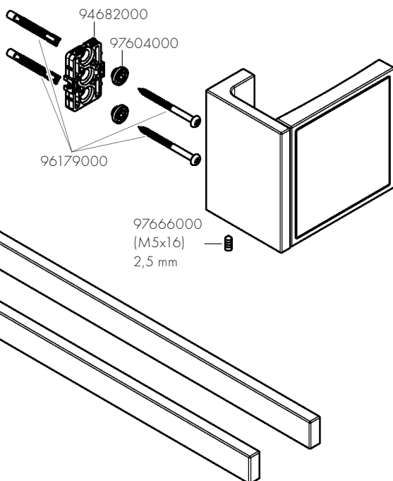
AXOR Universal Rectangular 42654XX0
