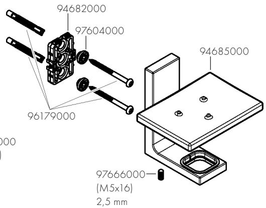
AXOR Universal Rectangular 42605XX0
