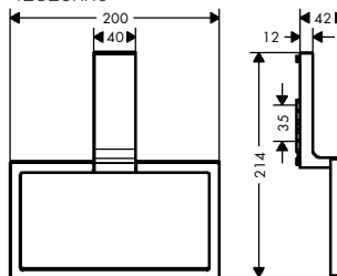
AXOR Universal Rectangular 42623XX0
