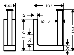
AXOR Universal Rectangular 42654XX0
