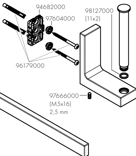
AXOR Universal Rectangular 42654XX0
