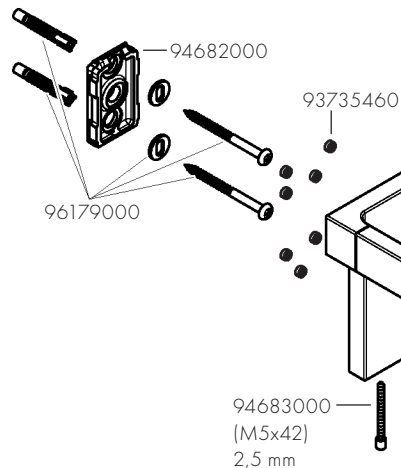
AXOR Universal Rectangular 42622XX0
