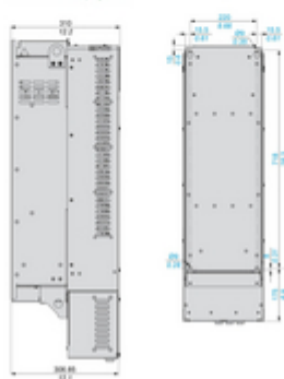
Drives Without IP21, Top Cover
