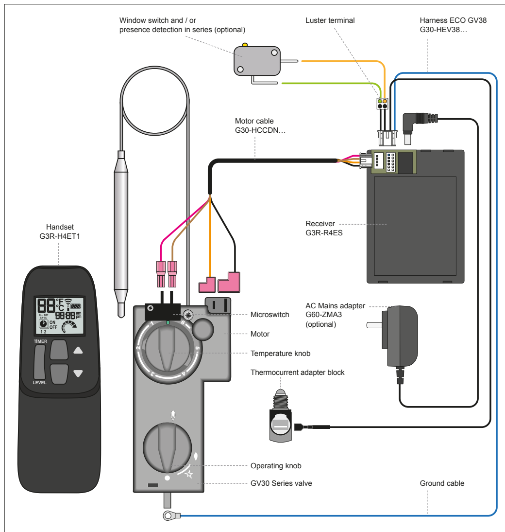
Figure 20: Wiring diagram
